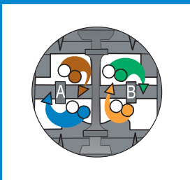
Adjust Pair Position for Cable End 2
