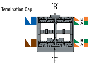
Pair Orientation for Cable End 1
