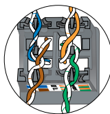
Pair Orientation for Cable End 2
